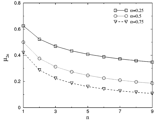
FIG. 1. In this figure the first few nonvanishing moments of P(m) are plotted for \alpha=1/4, 1/2 , and 3/4 .
